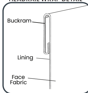
HEADRAIL WRAP DETAIL
